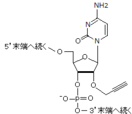
2'-O-propargyl rC
