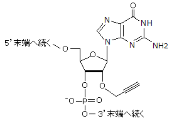
2'-O-propargyl rG
