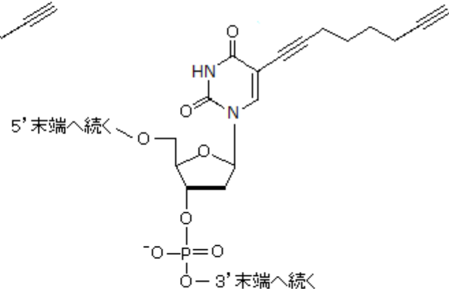
C8-alkyne-dU (5-Octadiynyl-dU)
