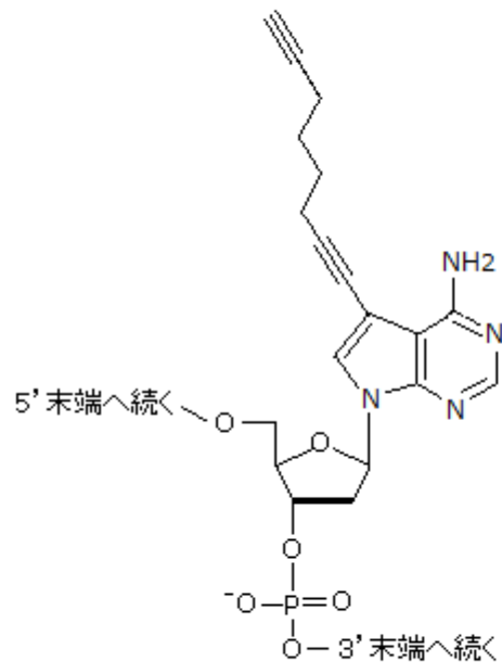
C8-alkyne-7-deaza-dA (7-Octadiynyl-7-deaza-dA)
